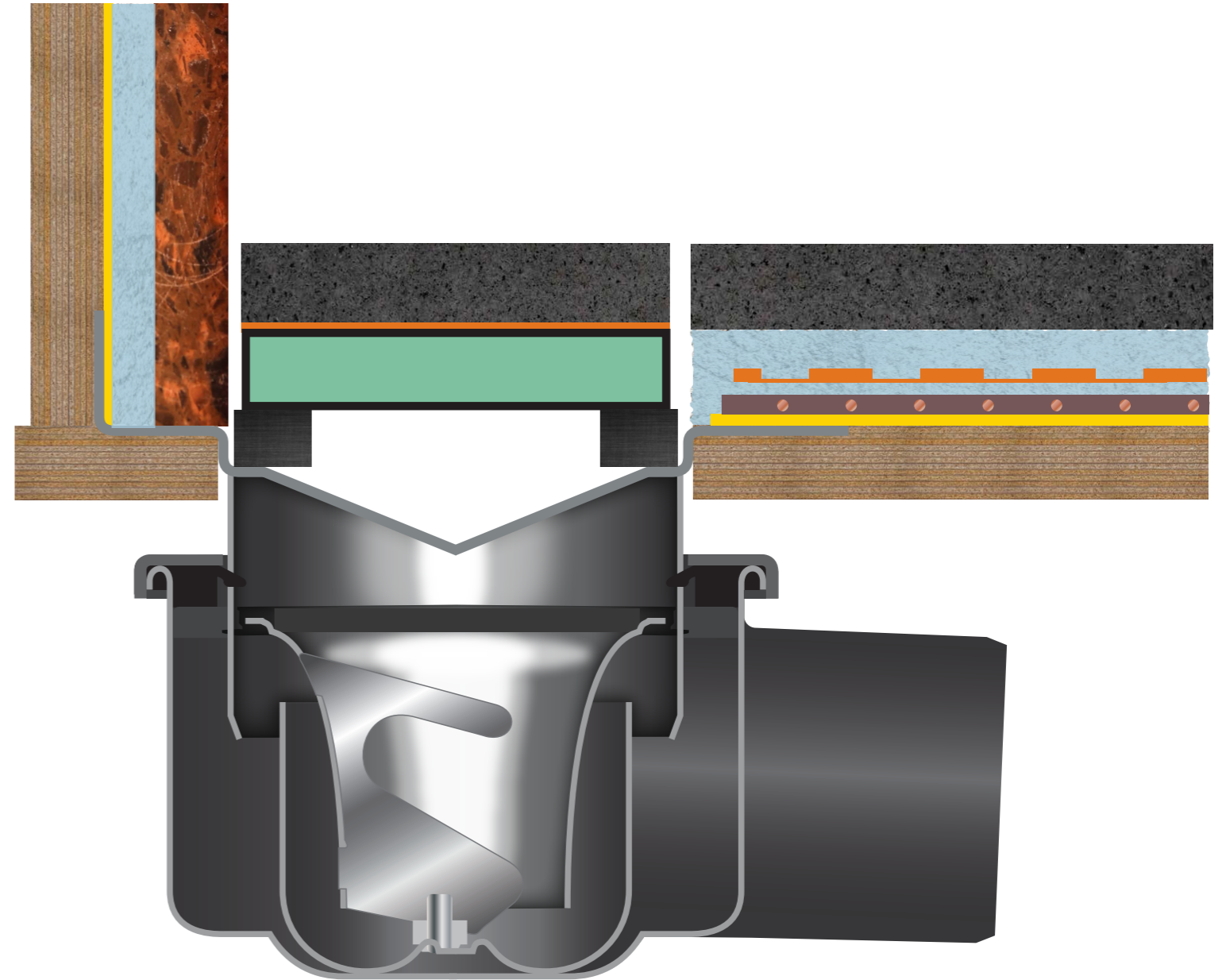
SECTION WITH TYPICAL FLOOR AND WALL BUILD UP
